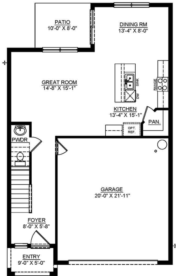
1ST FLOOR PLAN - ELEVATION G & H 8'-8" CLGS 03-31-2022
