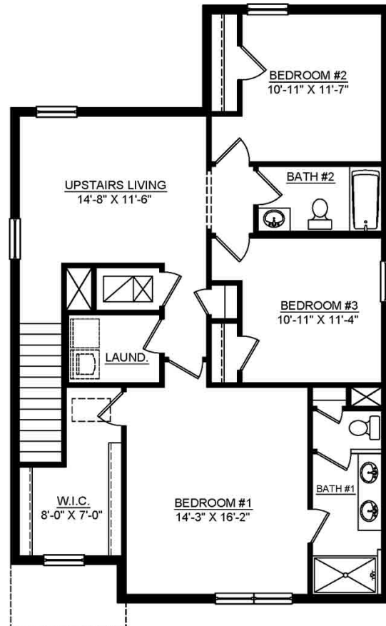
2ND FLOOR PLAN - ELEVATION G & H 8'-8" CLGS 03-31-2022
